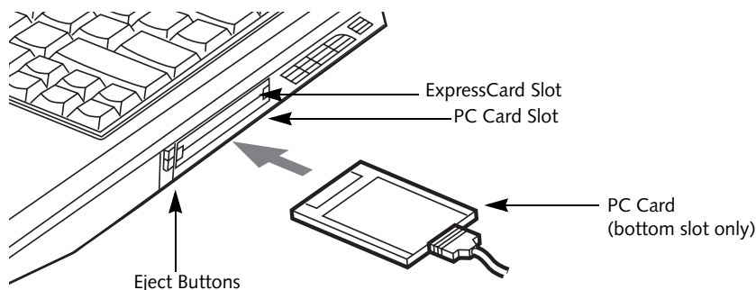
Figure 4-7. Installing/Removing PC Card
