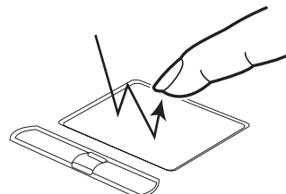
Figure 2-14 Double-clicking
