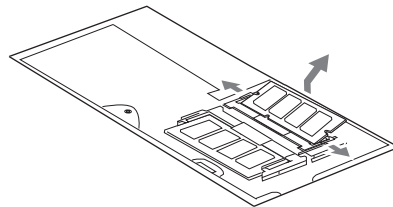
Figure 4-11. Removing a Memory Upgrade Module
