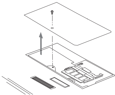
Figure 4-9. Opening the Memory Upgrade Compartment
