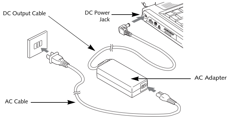
Figure 3-1 Connecting the AC Adapter
