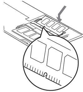
Figure 4-10. Installing a Second Memory Module
