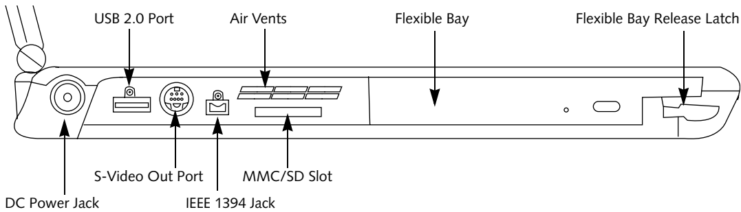
Figure 2-5. LifeBook notebook left-side panel
